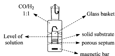
Figure 2. Special glass vial to be introduced into the high-pressure reactor for solid-liquid biphasic hydroformylation experiments.
