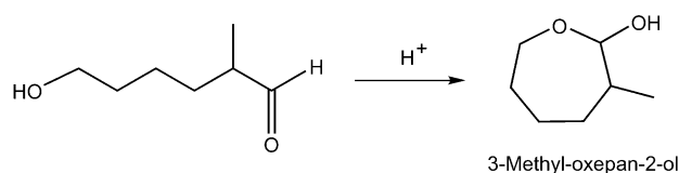
Scheme 4. Intramolecular cyclization of 6-hydroxy-2-methylhexanal.
