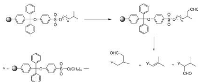
Scheme 1. First example of polymer-anchored alkene hydroformylation in a biphasic solid-liquid system.
