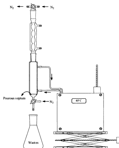
Figure 3. Apparatus to carry out solid phase reactions.
