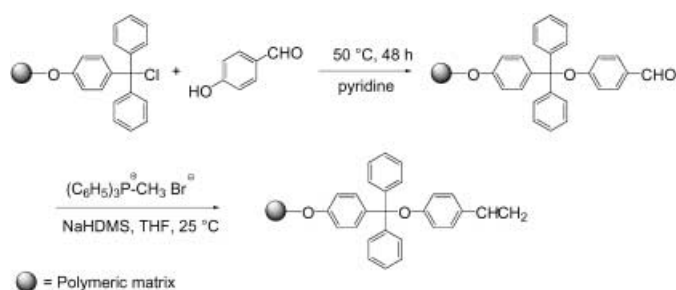
Scheme 3. Preparation of substrate 4 by Wittig reaction on solid phase.
