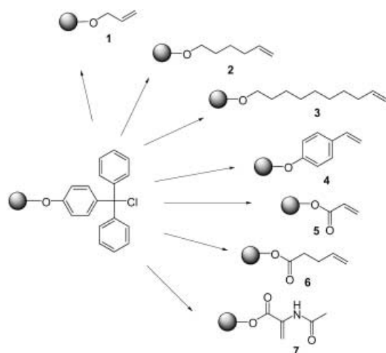
Figure 1. Substrates for biphasic solid-liquid hydroformylation using the trityl-derivatized polymeric support.
