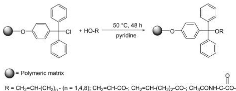
Scheme 2. Linking of various functionalized alkenes to a polymeric matrix.
